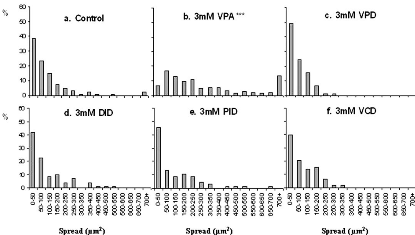
Fig. 3. Effects of VPA and aliphatic VPD constitutional isomers on rat DRGs growth cones spreading. The VPD constitutional isomers exhibit potent anticonvulsant activity in animal models of epilepsy (Table 1) (Haj-Yehia and Bialer, 1990; Winkler et al., 2005b). A histogram shows the percentage of growth cones with spread areas within 50- \mu\text{m}^2 class intervals. The abbreviations for the various compounds are given in Fig. 1. a, untreated control experiment, as shown in Fig. 2. b, 3 mM VPA-treated experiment, as shown in Fig. 2. c, 3 mM VPD-treated experiment, made up of 69 growth cones derived from three DRG explants. d, 3 mM DID-treated experiment, made up of 110 growth cones derived from three DRG explants. e, 3 mM PID-treated experiment, made up of 75 growth cones derived from four DRG explants. f, 3 mM VCD-treated experiment, made up of 60 growth cones derived from three DRG explants. Total data of a–f were analyzed by a Kruskal-Wallis test, followed by Dunn's multiple comparison test of each experiment versus control: ***, p < 0.001 .
